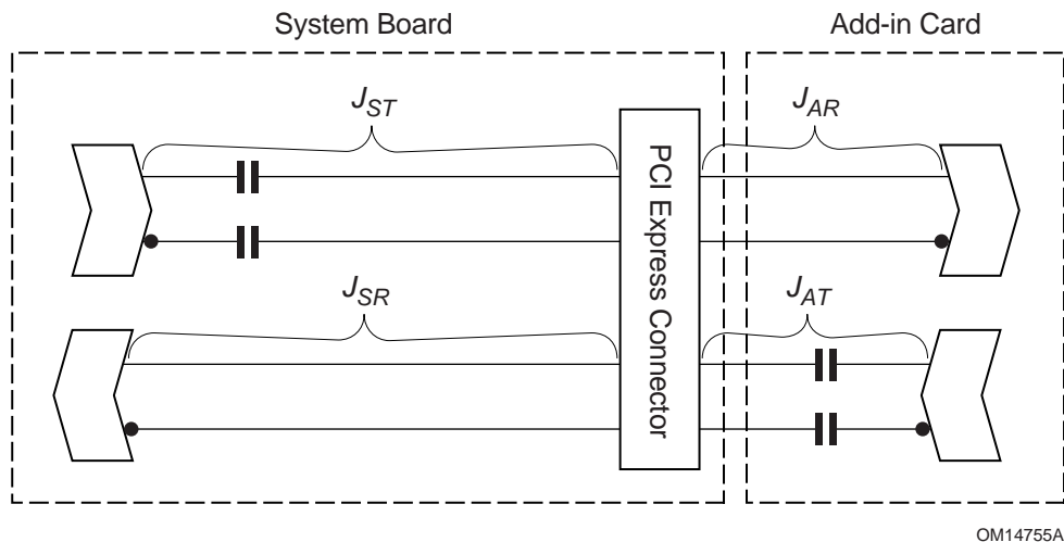
Figure 4-7: Jitter Budget
