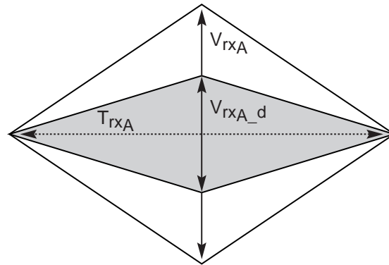
Figure 4-10: Representative Composite Eye Diagram for Add-in Card Receiver Path Compliance
