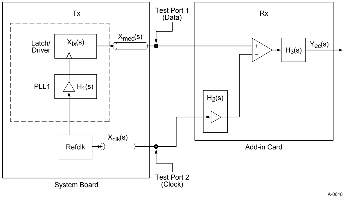
Figure 4-13: Two-Port Measurement Model
